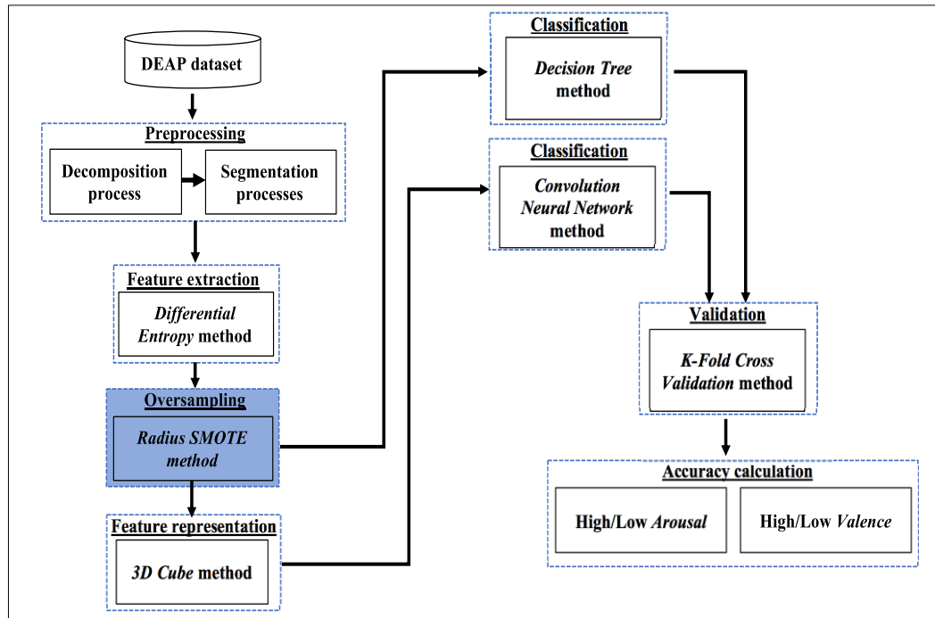
Figure 1. EEG signal-based emotion recognition flowchart
