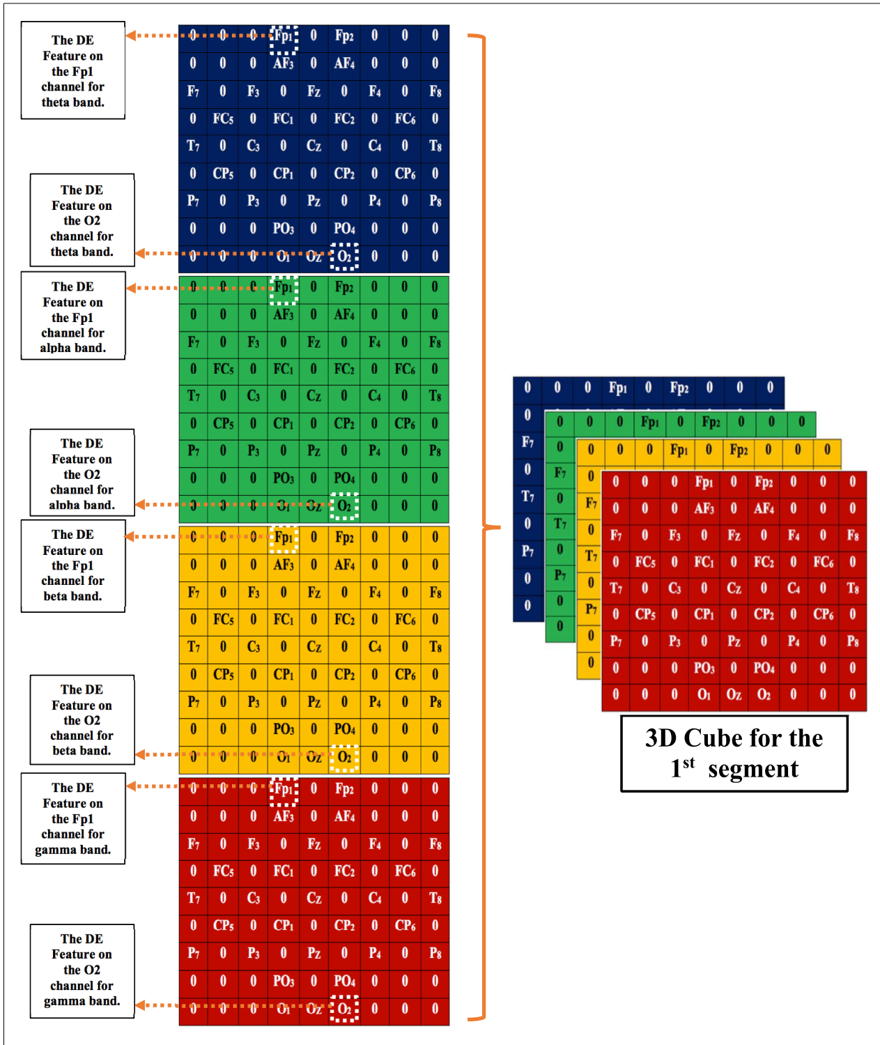
Figure 6. The feature representation using 3D Cube in one segment [46]
