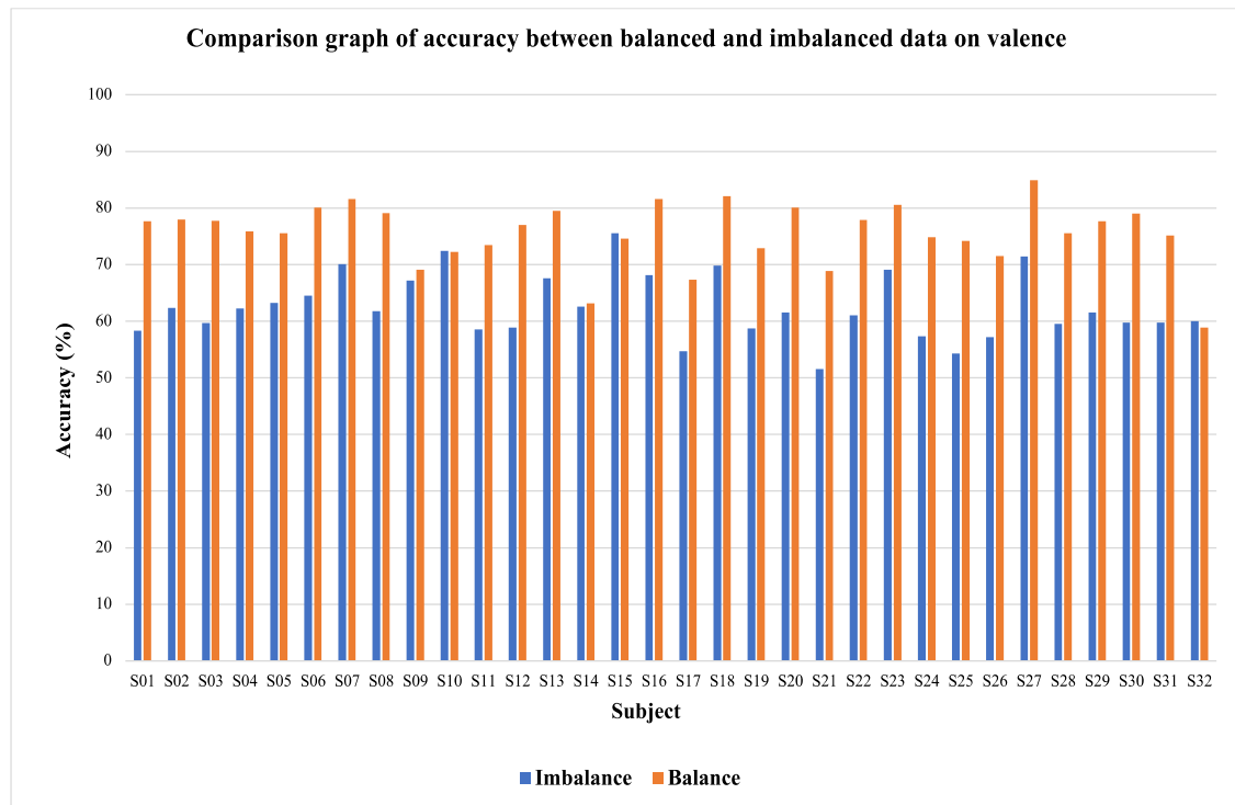
Figure 13. Comparison of valence accuracy for using Decision Tree and with or without the Radius SMOTE method
