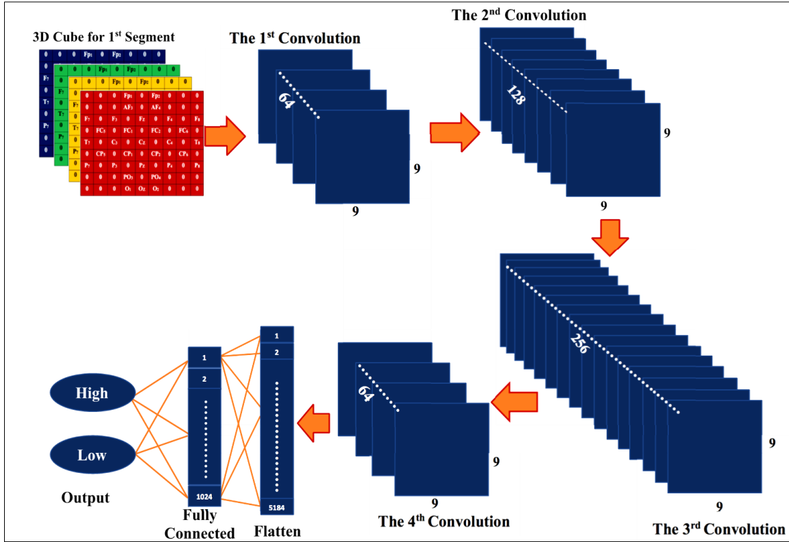
Figure 7. The classification process using CNN method for first 3D Cube [46]
